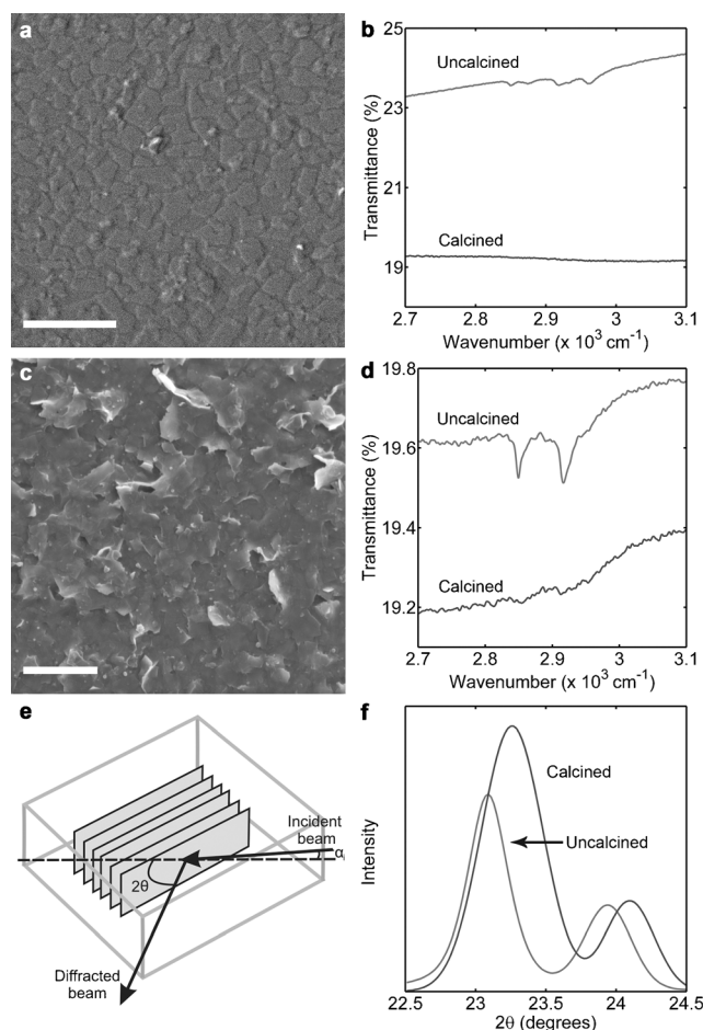
Figure 4. a, c) Single and multilayer nanosheet films made by LS; scale bars = 1 \mu m. b, d) FT-IR spectra obtained from nanosheet films similar to those displayed in (a, c), showing that the peaks corresponding to OSDA are absent after calcination. e) Schematic of in-plane X-ray diffraction, where \alpha is the angle of incidence and 2\theta is the angle between the incident beam and the detector. f) In-plane X-ray diffraction patterns obtained from a multilayer nanosheet film showing that there is in-plane contraction of the crystalline framework caused by OSDA removal on calcination.
